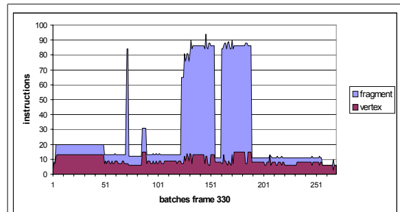
Figure 6. Vertex and fragment program instructions for frame 330.
